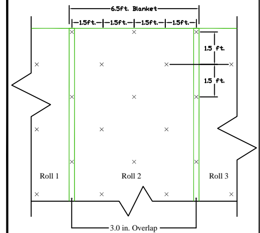
Figure D - Plan View × - Denotes Staple Locator
